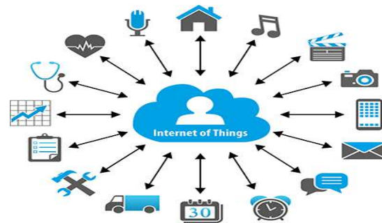
Fig 1:IoT Applications
